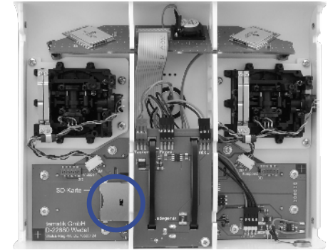
SD Card slot in the radio
